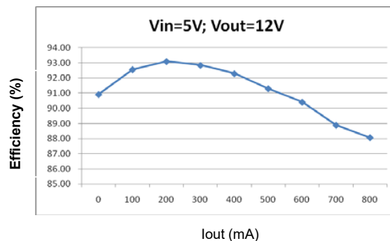
Figure 2. Efficiency Curve
